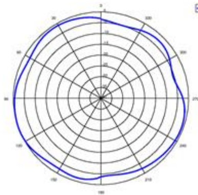
2.4G (Horizontal)
